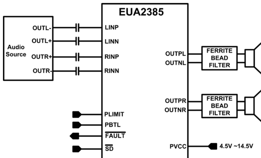
Figure1. Simplified Application Schematic
